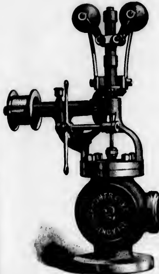
Class "B," SPRING GOVERNOR WITH SPEEDER AND SAWYER'S LEVER, AND WITH OR WITHOUT AUTOMATIC SAFETY STOP
